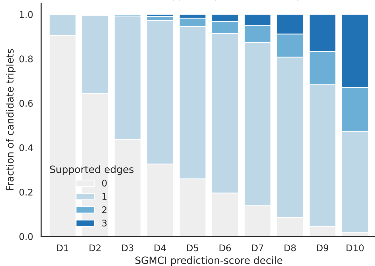
Number of supported pairwise Hi-C edges
