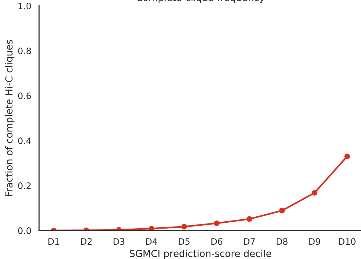
Complete-clique frequency
